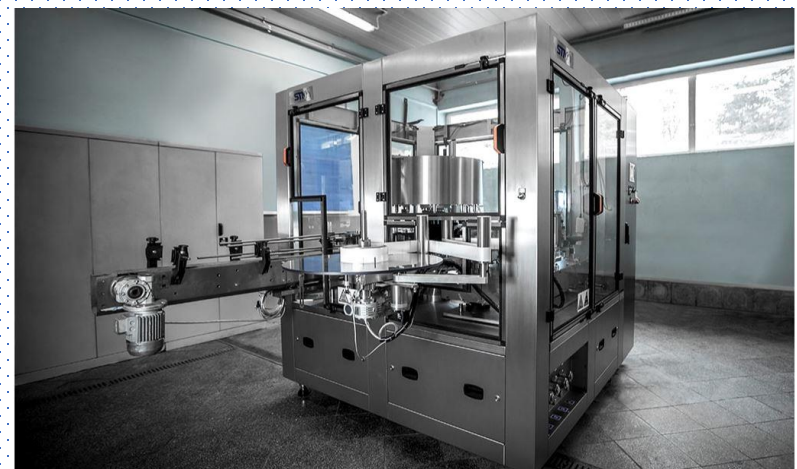
Labeling Machine
